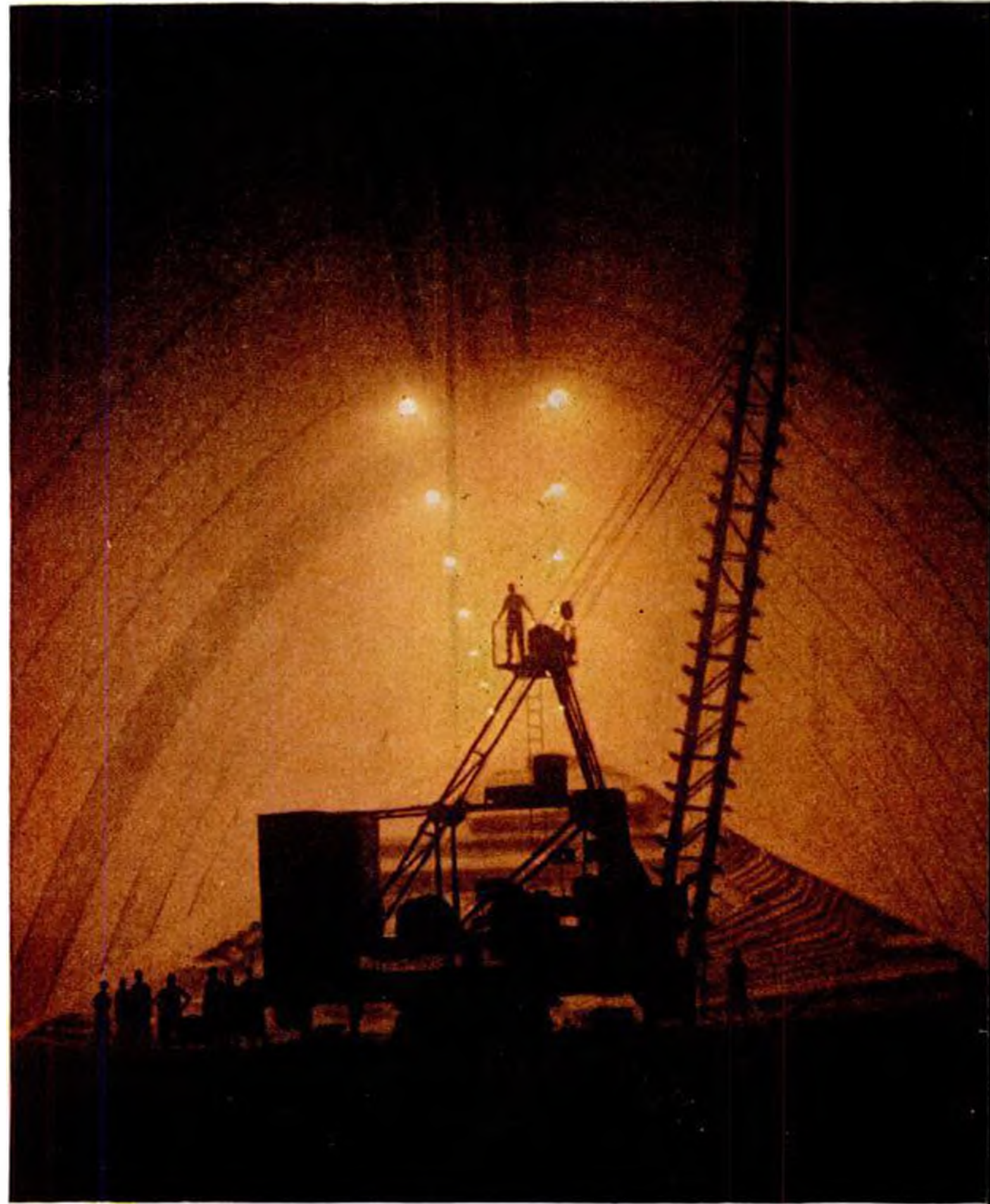
LOADING FERTILIZER at Sindri, crane scoops up ammonium sulfate, moving it out of the storage silo. Ultramodern Sindri plant employs 3,500 people.
