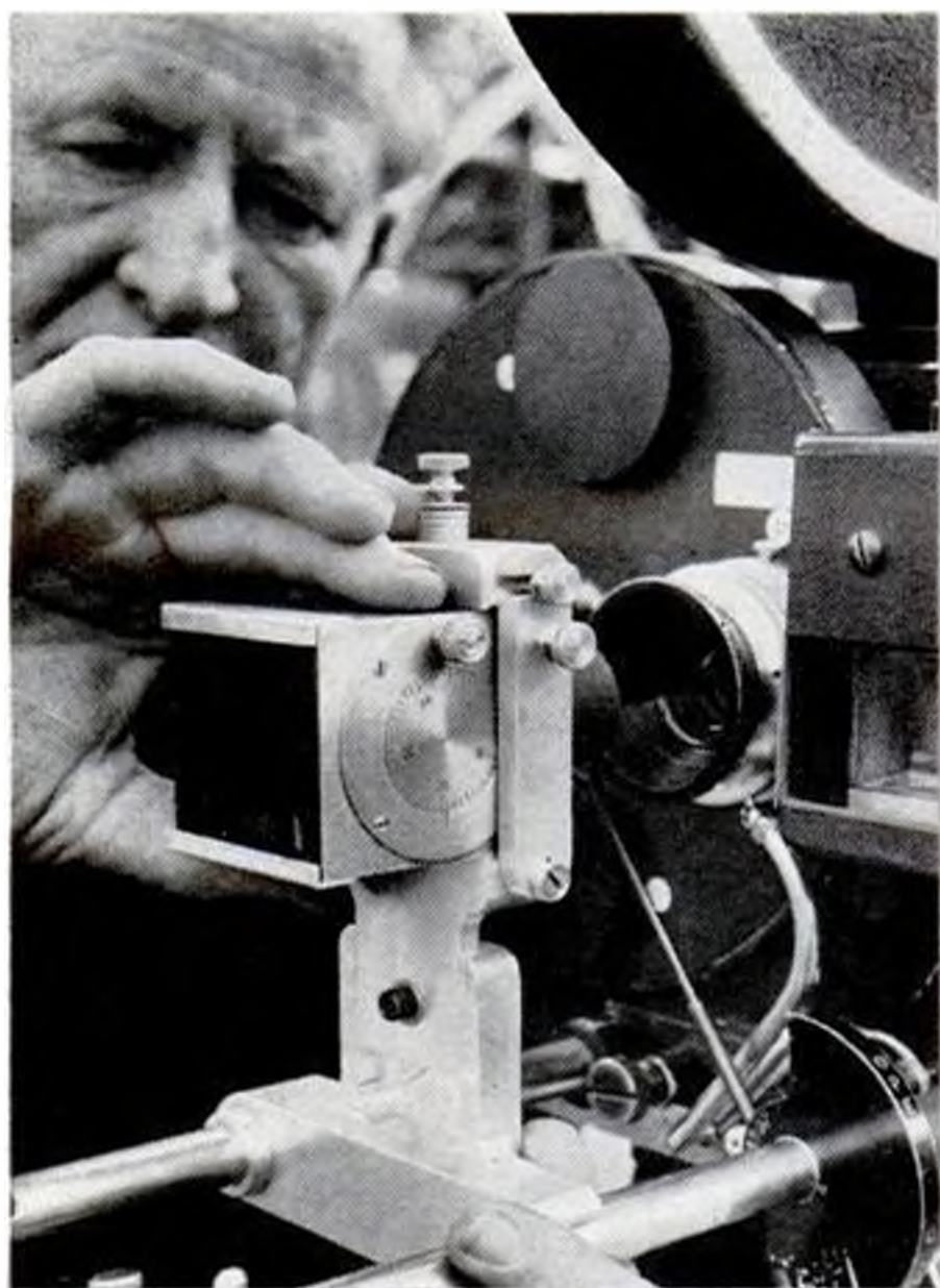
SECRET of Cinemascope is device called anamorphoser, perfected by Frenchman Henri Chrétien in 1931, which squeezes wide image onto 35-mm film.
